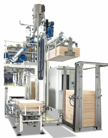
■ Robo XI: automatic robot for the end-of-line
